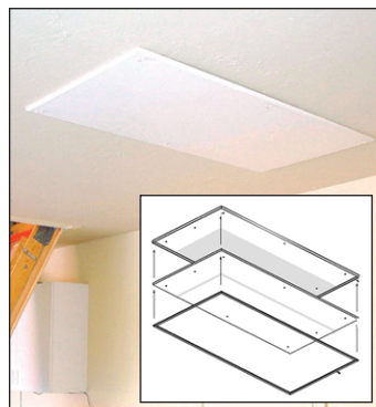
Fire Rated Ceiling Panel
