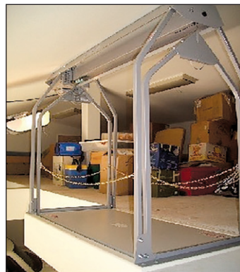
Cantilever installation
